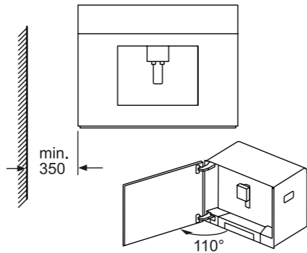
Left corner installation
